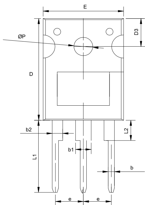
TO-3P
