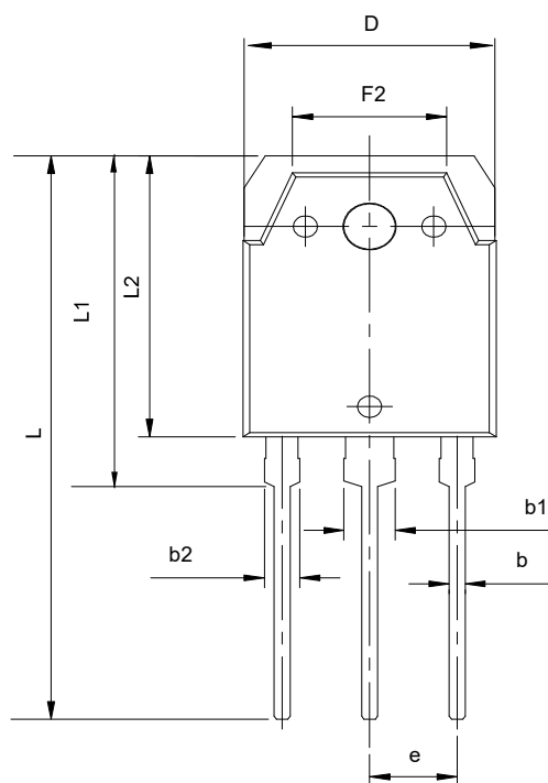
TO-3P
